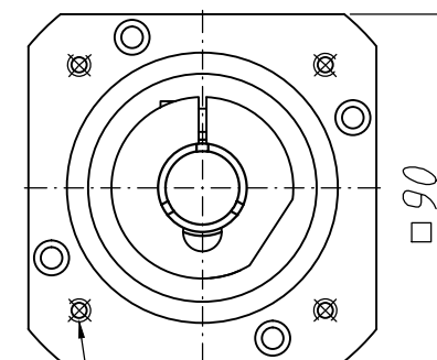
4-M6XP1 PCD \phi 90
