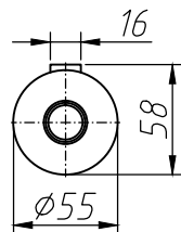
Output shaft
