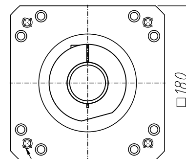
4-M12xP1.75 PCD \phi 200
