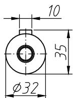
Output shaft
