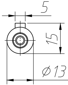
Output shaft
