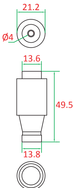
E-27 Fuse
