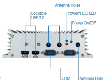
Front Panel External I/O
