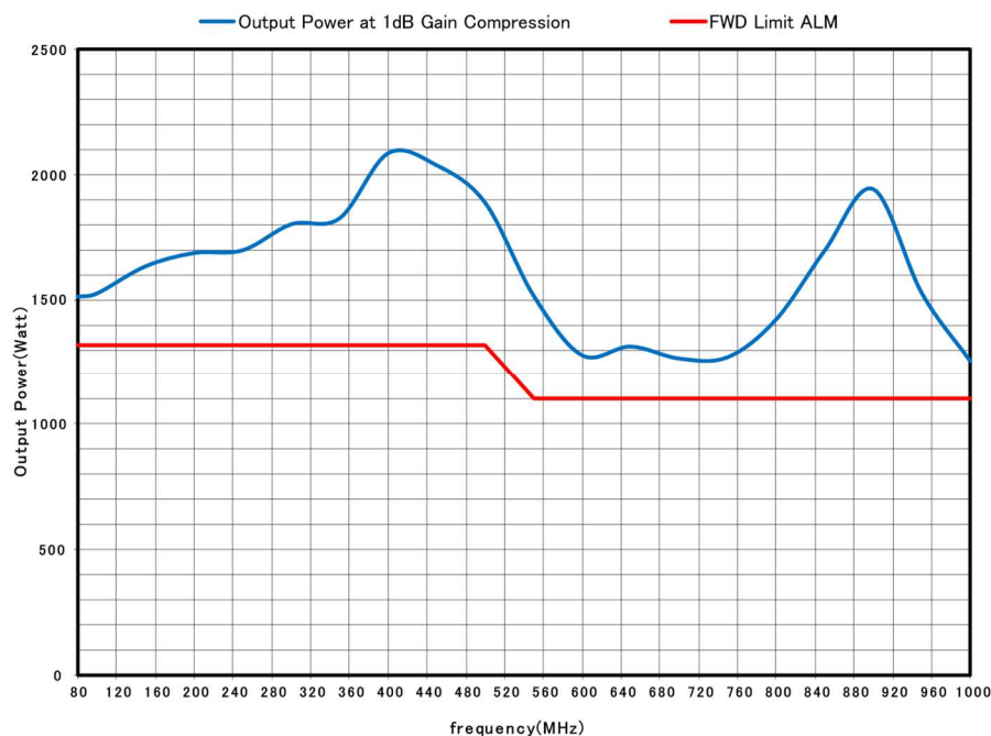
Model ZSA6161-80M1GA Typical Power Output
