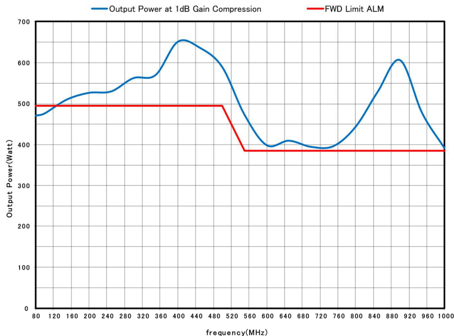
Model ZSA5656-80M1GA Typical Power Output
