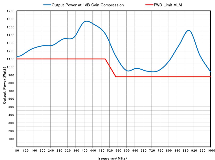
Model ZSA6060-80M1GA Typical Power Output
