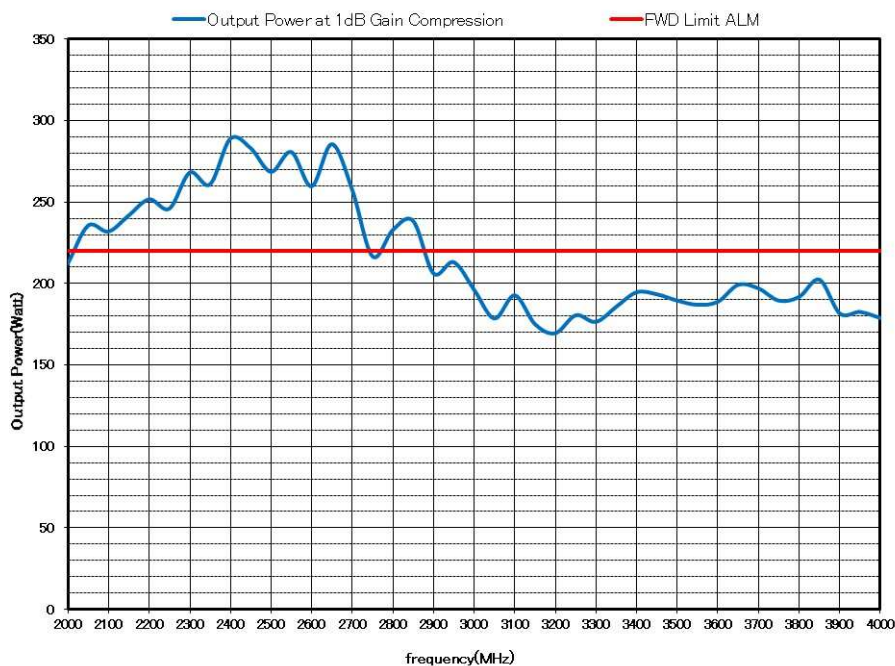
Model ZSA5353-2G4G Typical Power Output
