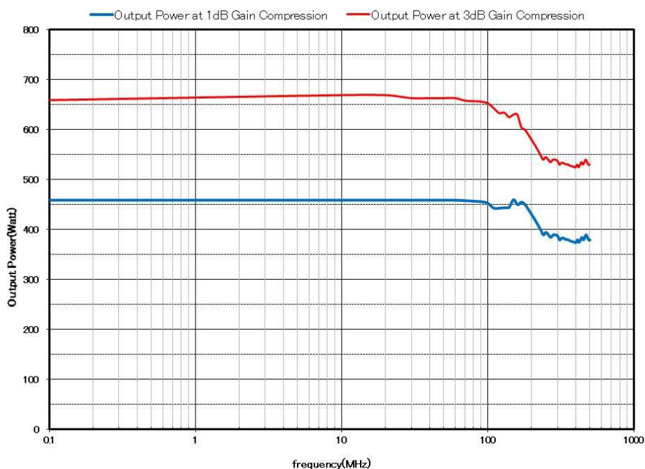
Model ZSA5757-100K500M Typical Power Output
