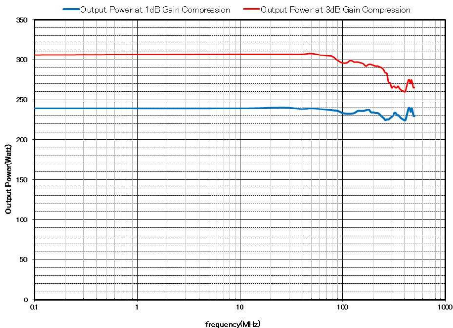
Model ZSA5454-100K500M Typical Power Output
