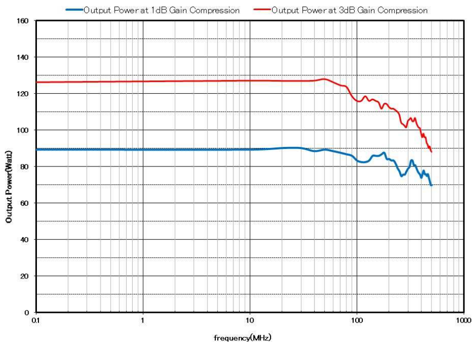
Model ZSA4949-100K500M Typical Power Output
