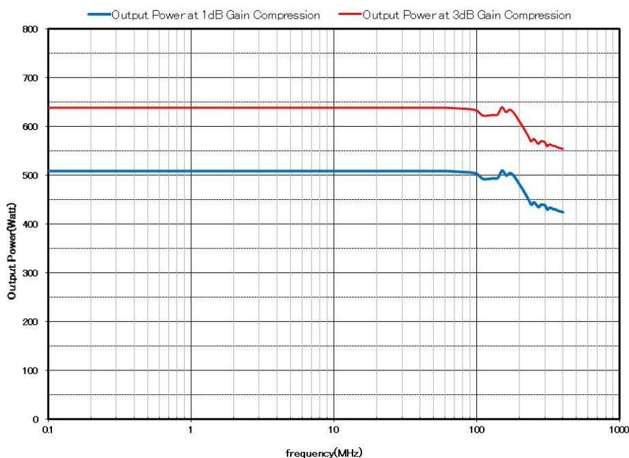
Model ZSA5757-100K400M Typical Power Output
