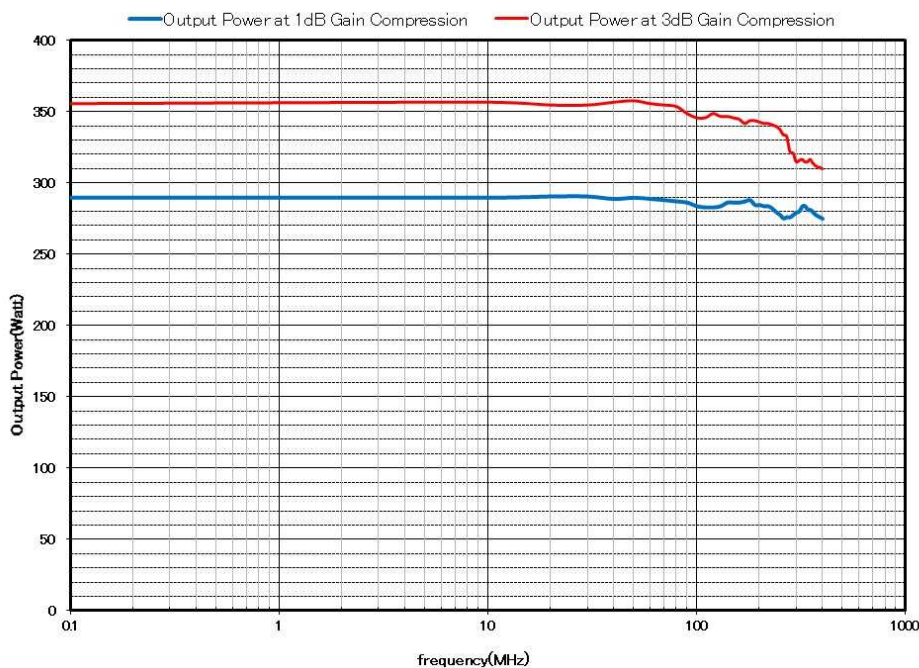
Model ZSA5555-100K400M Typical Power Output
