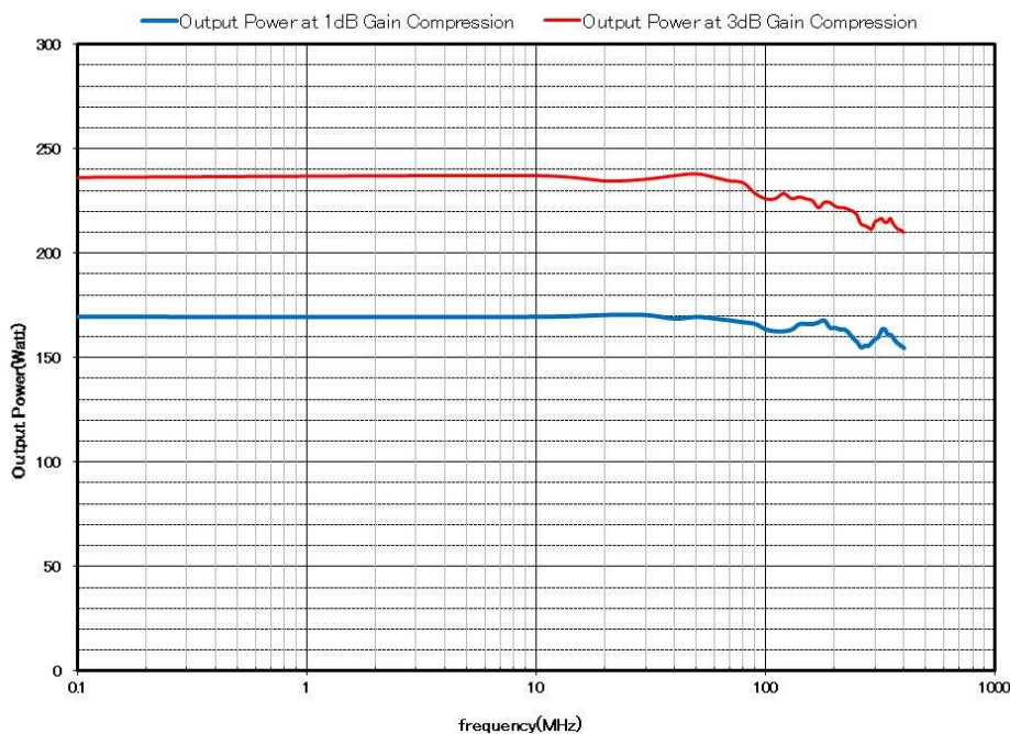
Model ZSA5353-100K400M Typical Power Output
