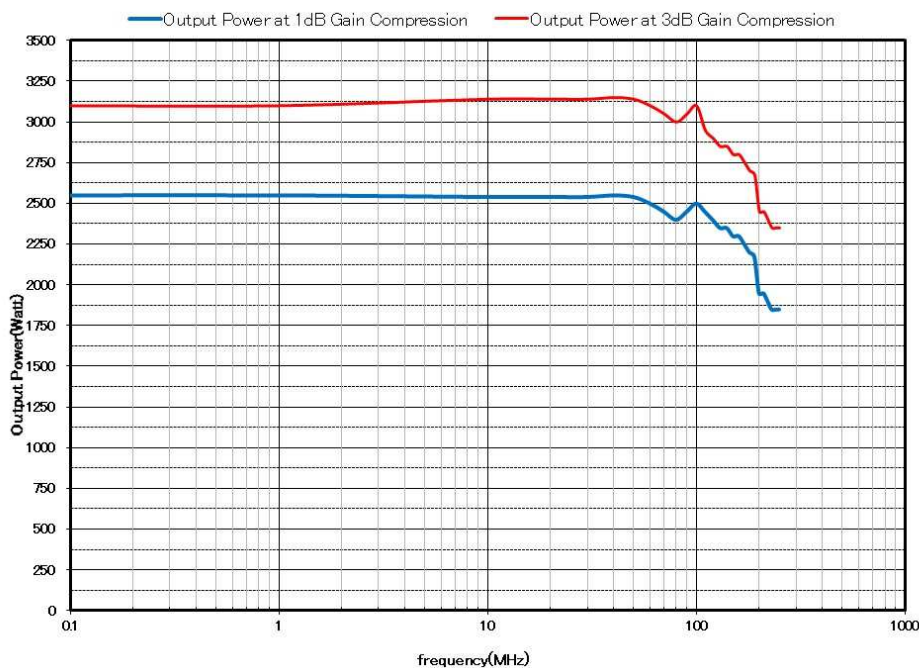
Model ZSA6363-100K250M Typical Power Output
