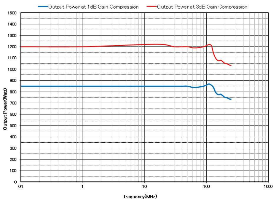
Model ZSA6060-100K250M Typical Power Output
