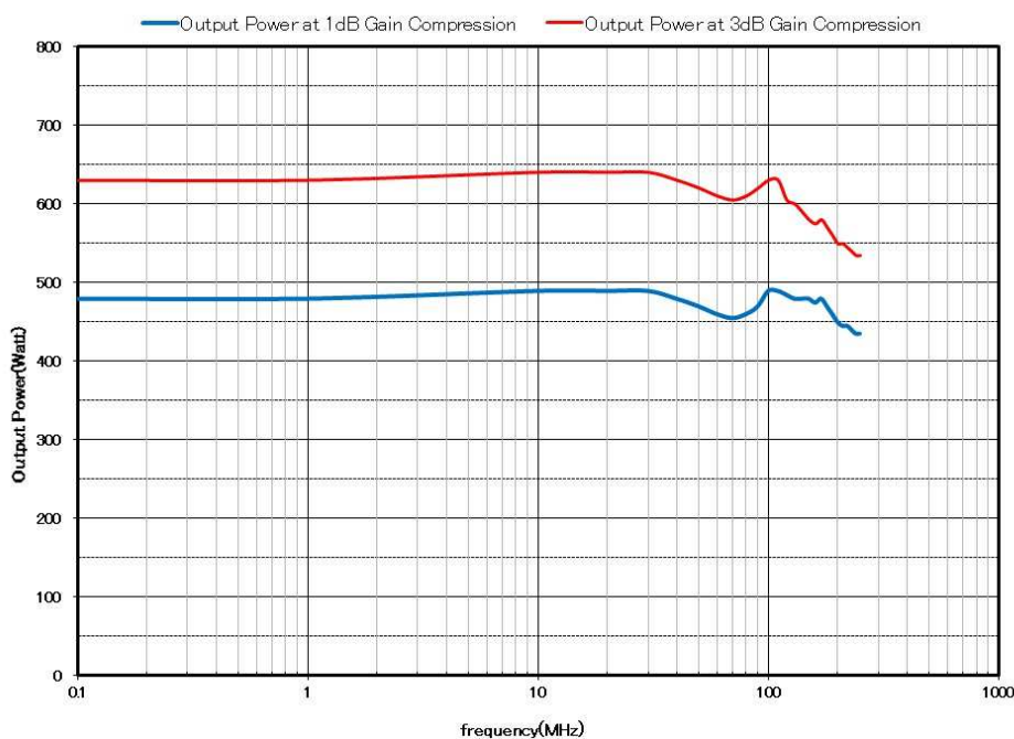
Model ZSA5757-100K250M Typical Power Output
