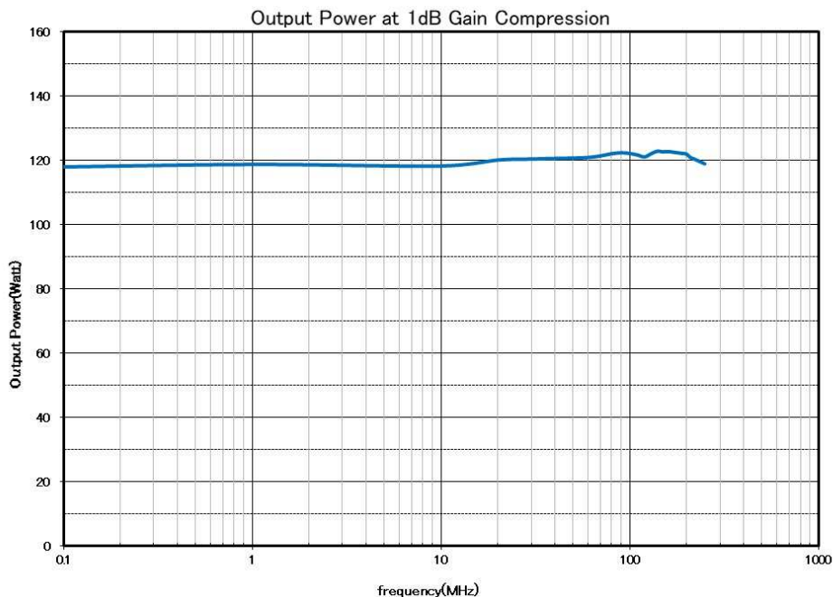
Model ZSA5050-100K250M Typical Power Output
