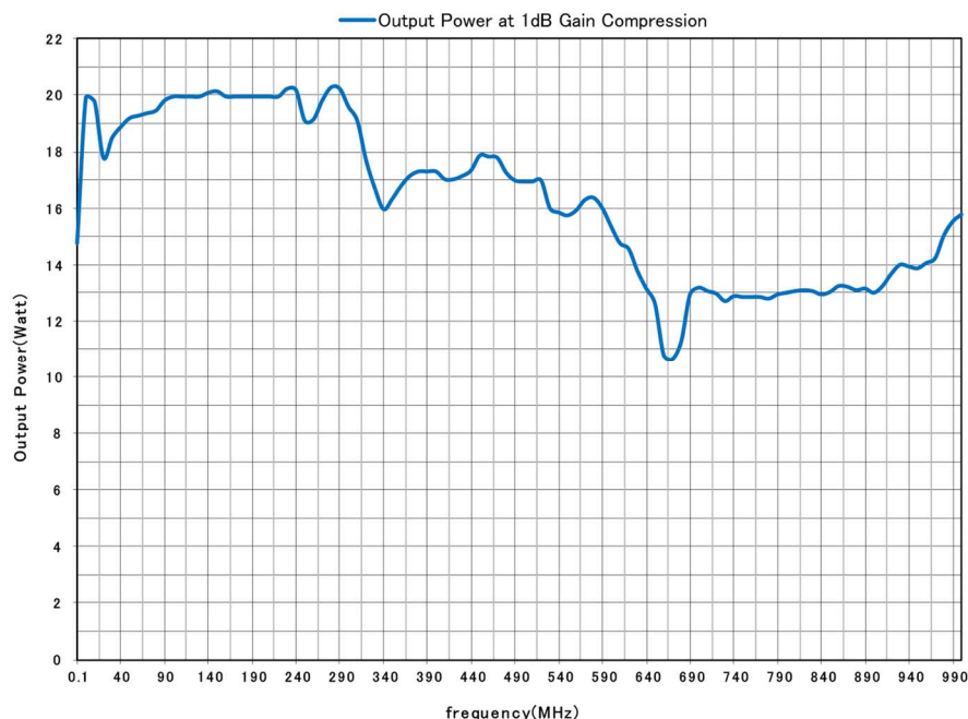
Model ZSA4040-100k1GA Typical Power Output
