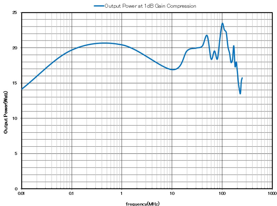
Model ZSA4242-10K250M Typical Power Output
