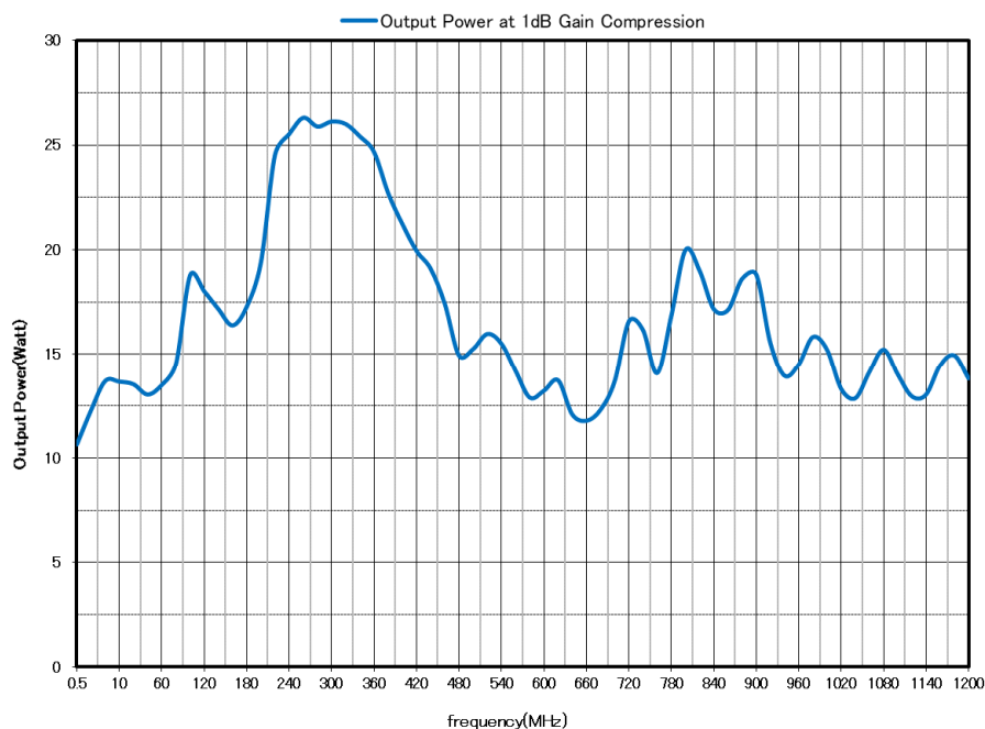
Model ZSA4040—500K1.2G Typical Power Output
