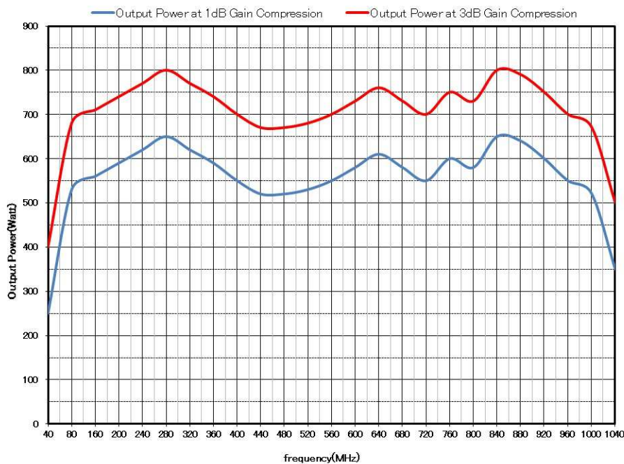
Model ZSA5858-80M1G Typical Power Output
