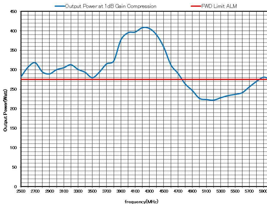
Model ZSA5454–2500M6G Typical Power Output
