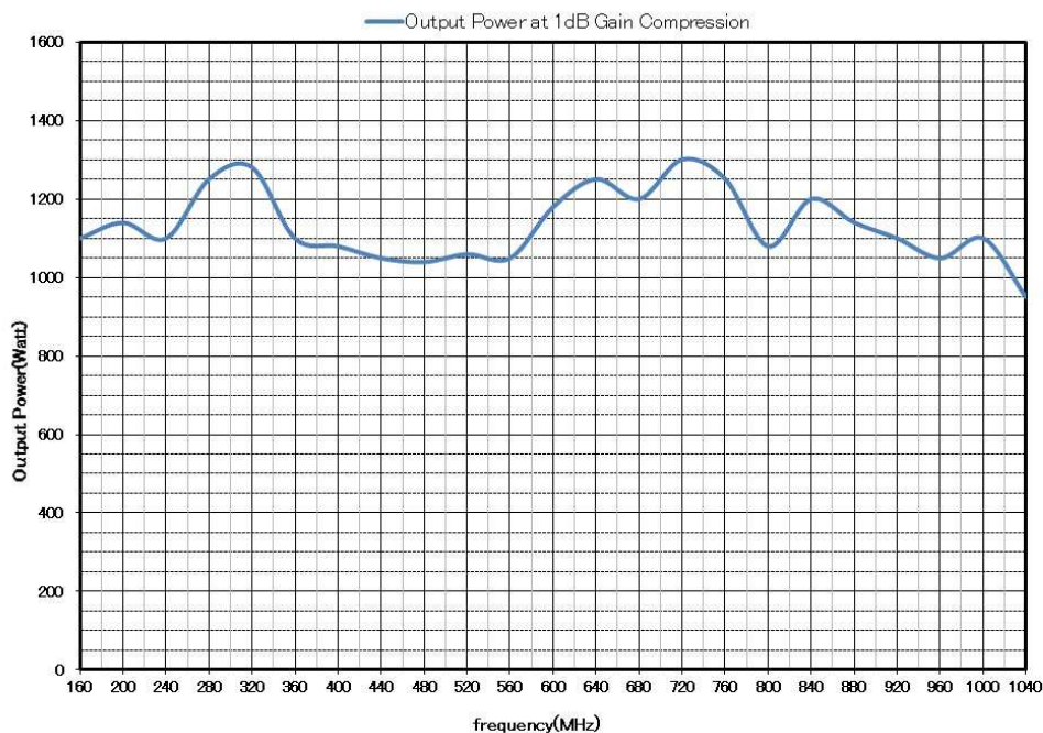
Model ZSA6060–200M1G Typical Power Output
