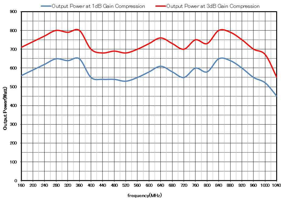
Model ZSA5858-200M1G Typical Power Output
