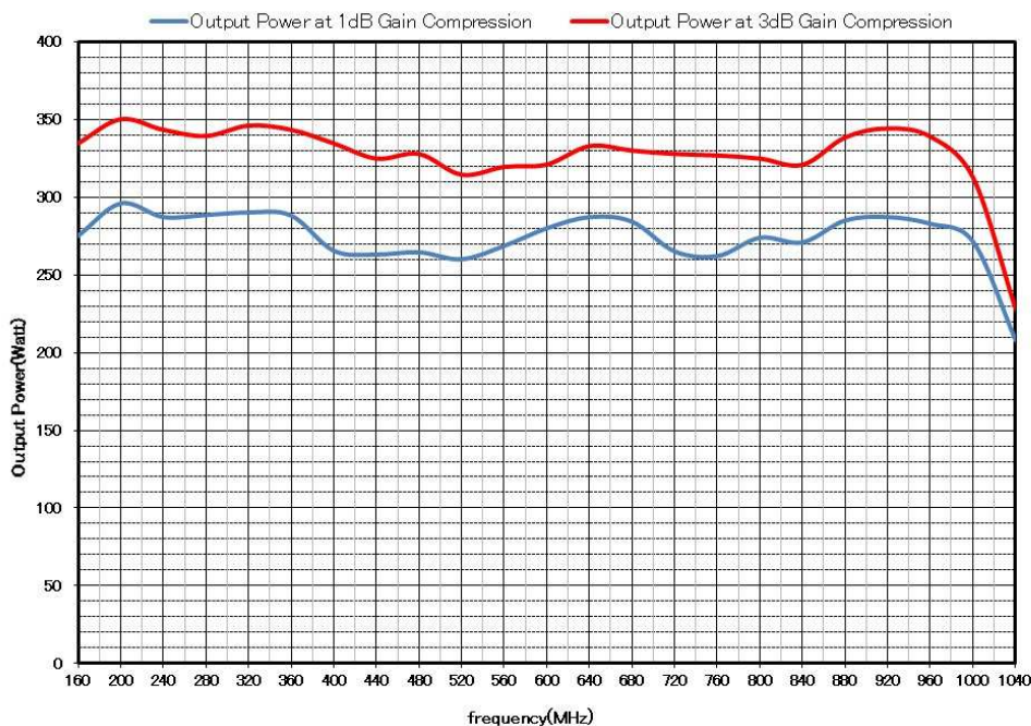
Model ZSA5555-200M1G Typical Power Output
