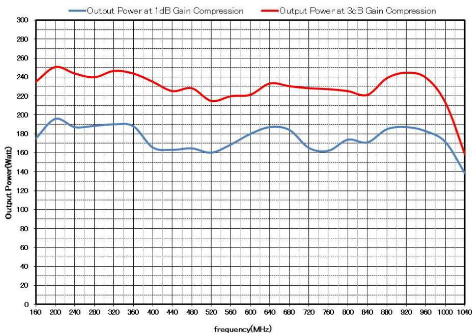
Model ZSA5353-200M1G Typical Power Output
