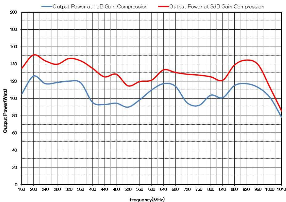
Model ZSA5050-200M1G Typical Power Output
