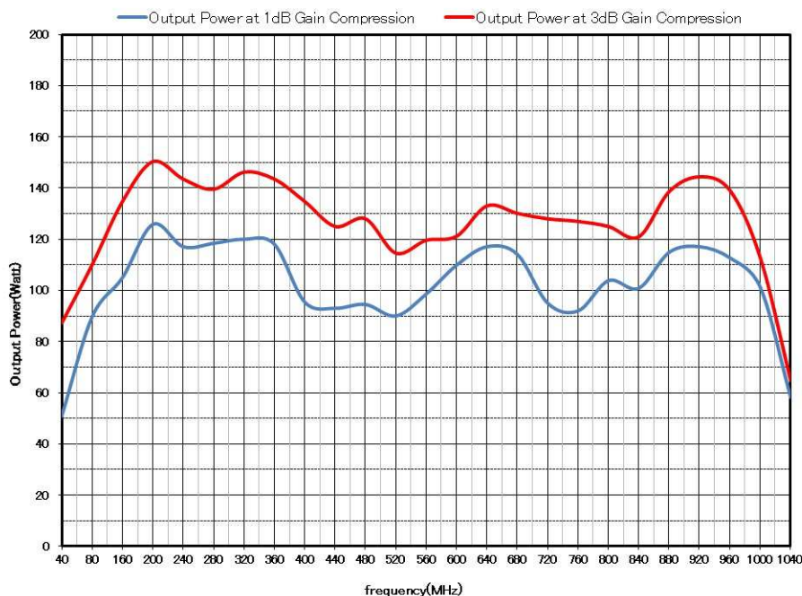
Model ZSA5050-80M1G Typical Power Output
