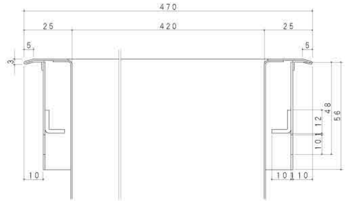
AA断面(1/1)
