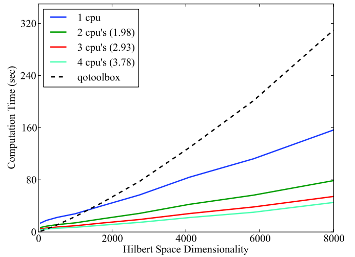
Fig. 12. (Color online.) Comparison of computation times, averaged over three runs, between QuTiP and the qotoolbox (dashed) in simulating the trilinear Hamiltonian from Eq. (18) for an initial pump mode coherent state with expectation value \langle N \rangle_a = \sqrt[3]{D}/4 as a function of the Hilbert space dimensionality D . The average performance enhancement from using multiple processors, as compared to the single-processor performance, is given in the legend. Ideally, this value should be equal to the number of processors. Computations were performed on a quad-core 2.8 GHz processor.
